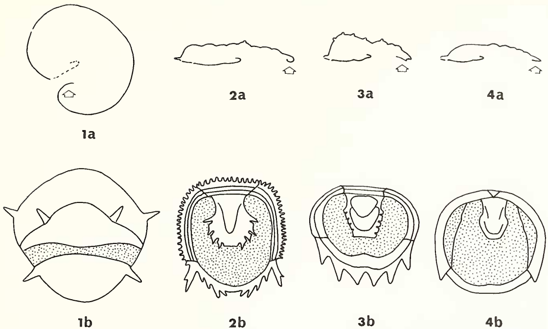
TEXT-FIG. 9. Sagittal sections (a) and ventral views (b) of four protaspids to show 'enrolled' (1), 'incurved' (2), and 'inturned' doublure (3, 4). For scale, see text-figs. 10 and 11. The open arrows point towards the protopygidial doublure. 1, Remopleurides sp. aff. R. eximius Whittington (Middle Ordovician, Edinburg Formation, Virginia). 2, Flexicalymene senaria? (Conrad) (Middle Ordovician, Martinsburg Shale, Virginia). 3, Acanthopyge bifida Edgell (Lower Devonian, Receptaculites Limestone, nr. Yass, New South Wales). 4, Proetus talenti Chatterton (Lower Devonian, Warroo Limestone, nr. Yass, New South Wales).
